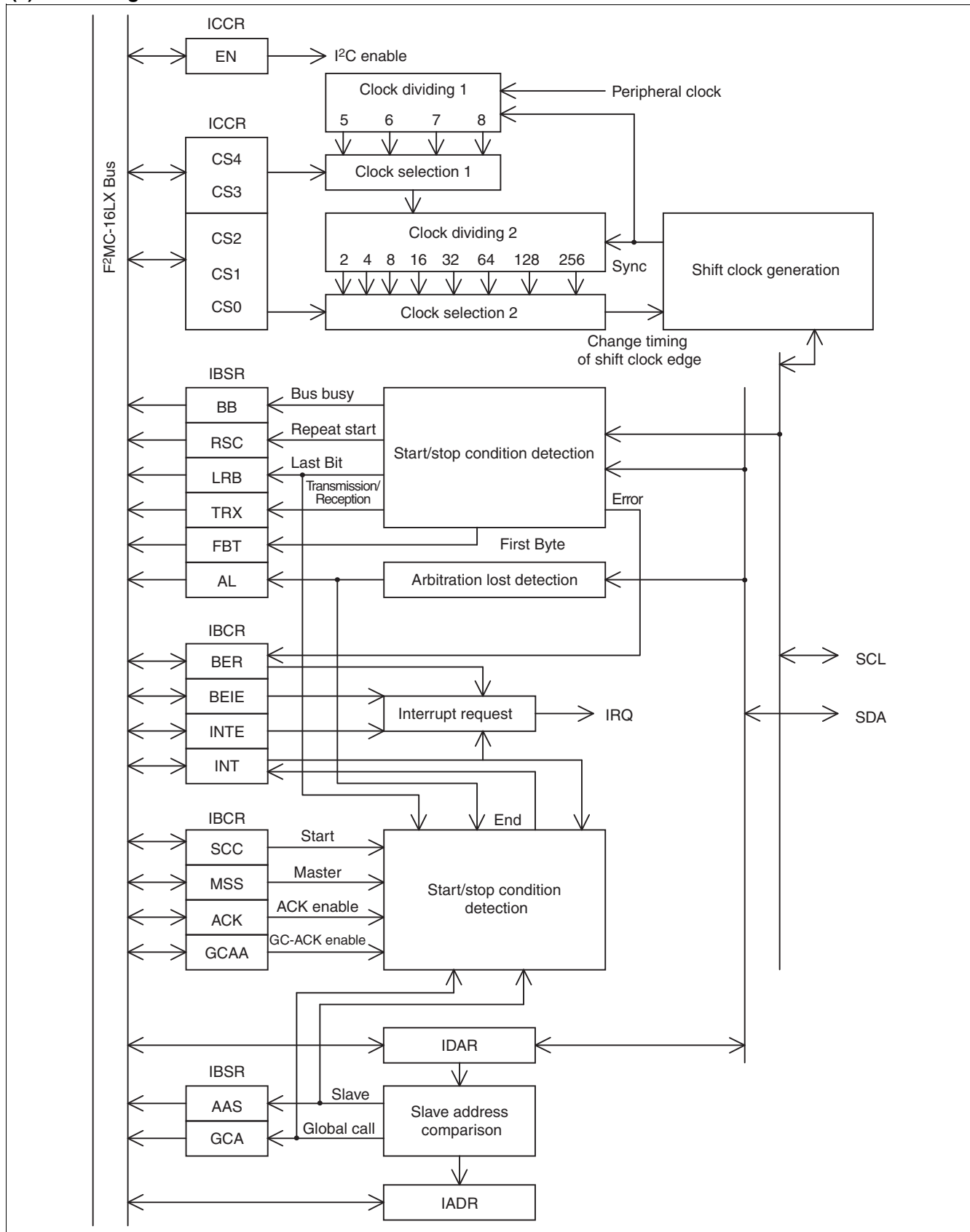
(2) Block Diagram
