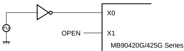
Sample external clock connection
