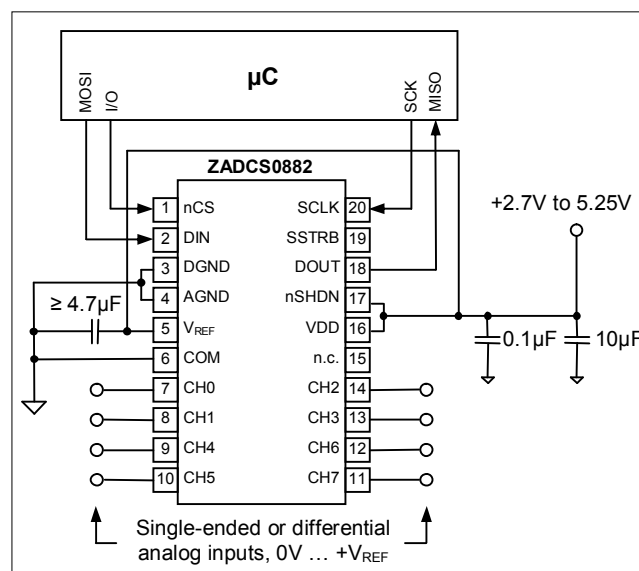
Figure 5: Basic application schematic for ZADCS0882
