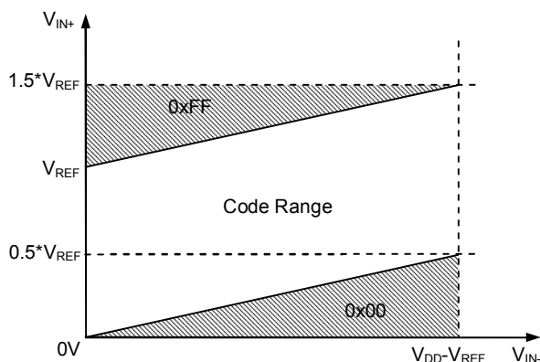
Figure 8: Input voltage range in unipolar mode
