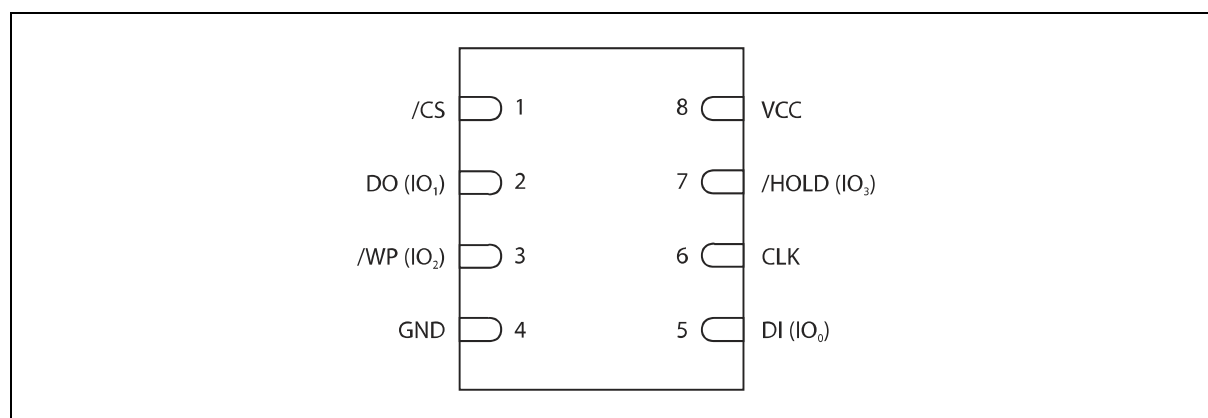
Figure 1b. W25Q32BW Pad Assignments, 8-pad WSON (Package Code ZP & ZE)
