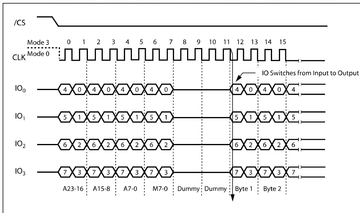
Figure 13b. Fast Read Dual I/O Instruction Sequence (Previous instruction set M5-4 = 10)
