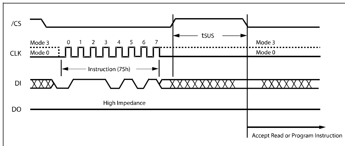
Figure 24. Erase/Program Suspend Instruction Sequence
